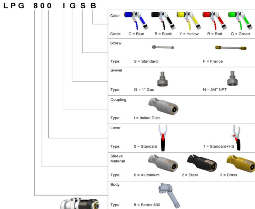
NOZZLE EXAMPLE MODEL LPG 800 IGSB
